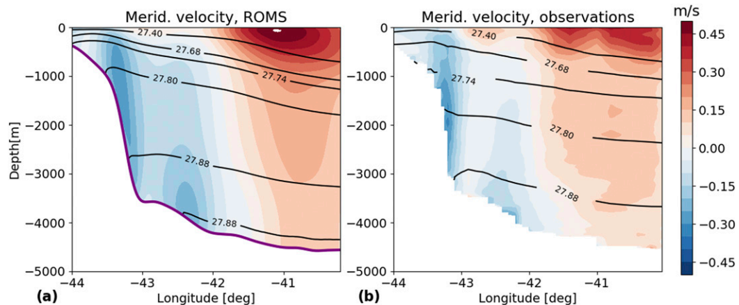
FIG. B2. Vertical section of meridional (approximately along-slope) velocity east of Flemish Cap (FC) along 47^\circ\text{N} , in (a) ROMS (year 16 average) and (b) 6-repeat ship ADCP observations after M14. Section location is marked by the red line east of FC in Fig. 1.
