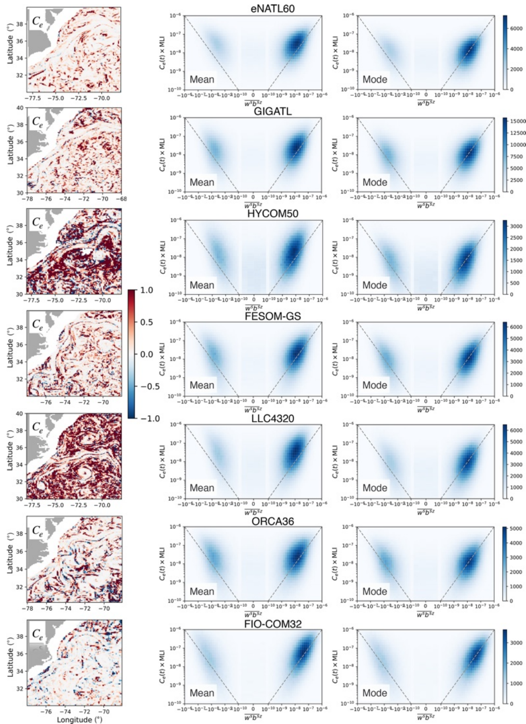
Figure E1. Snapshot of the efficiency coefficient C_e(t, x, y) diagnosed on 1 February from each simulation (left column). The joint histogram of \langle \overline{w^s b^z} \rangle and C_e(t) \times \text{MLI} during the months of February to April (right columns). The middle column shows the histogram when C_e(t) is taken as the spatial mean of C_e(t, x, y) and the right column as the spatial mode of C_e(t, x, y) . The one-to-one line is shown as the grey dashed line.
